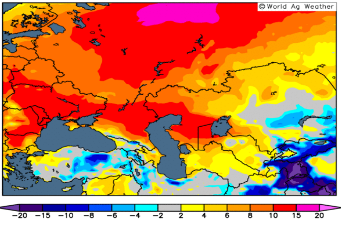
GEFS Ensemble Mean Temperature Anomaly (°F) Days 1-7: 00UTC 15 Feb 2022 – 00UTC 22 Feb 2022 Model Initialized 00UTC 14 Feb 2022
