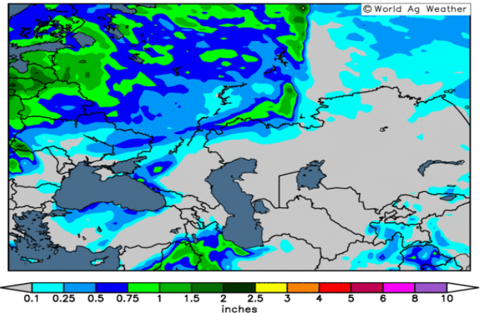
GFS High-Resolution Precipitation Forecast Days 1-7: 00UTC 15 Feb 2022 – 00UTC 22 Feb 2022 Model Initialized 00UTC 14 Feb 2022
